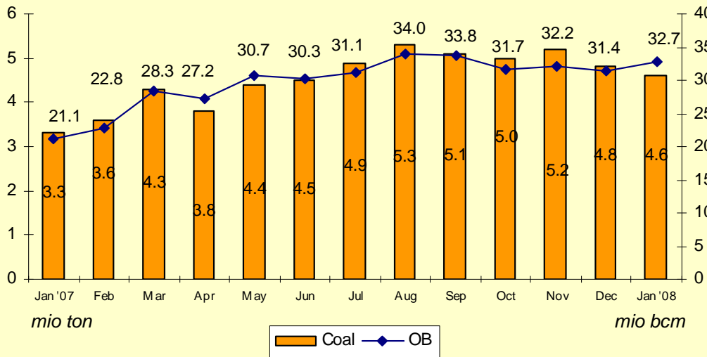
Historical Coal Production & Overburden Removal
