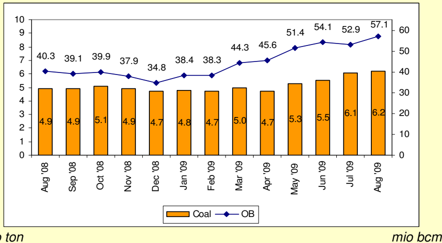
Historical Coal Production & Overburden Removal
