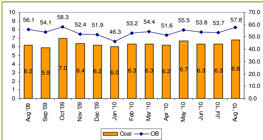
Historical Coal Production & Overburden Removal
