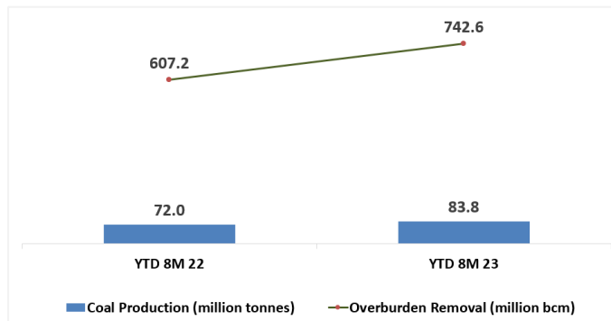
Coal Production and Overburden Removal
