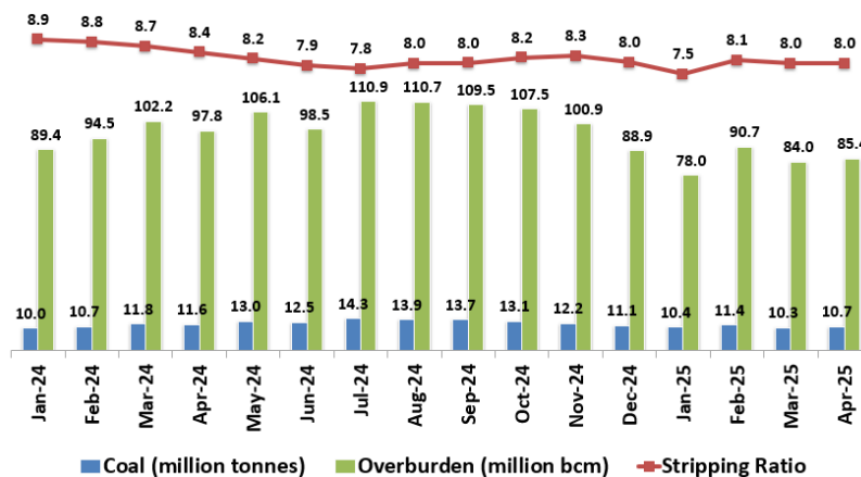
Monthly Coal Production and Overburden Removal
