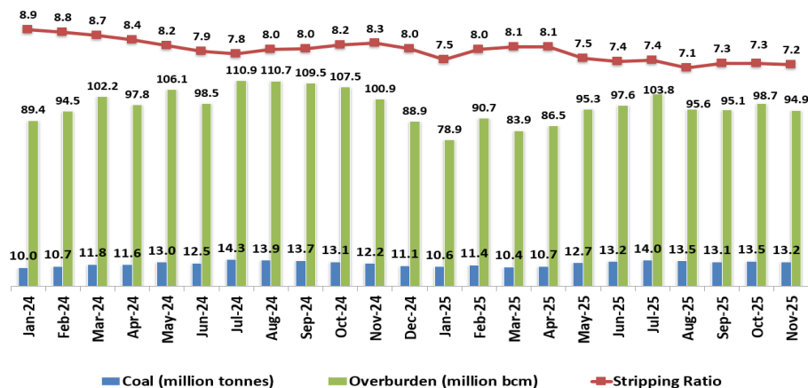
Monthly Coal Production and Overburden Removal
