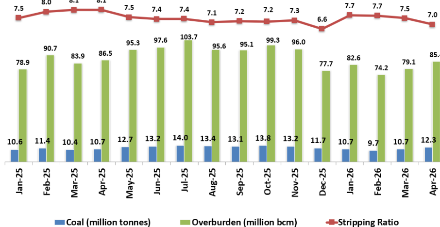
Monthly Coal Production and Overburden Removal
